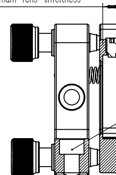
Cross section A-A
