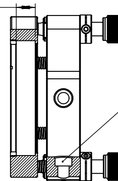
Cross section C-C
