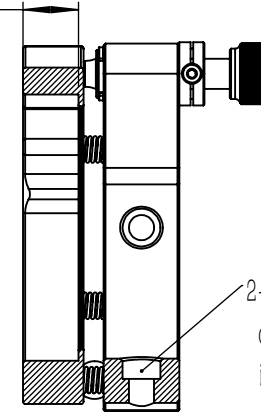
Cross section C-C
