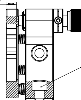
Cross section C—C
