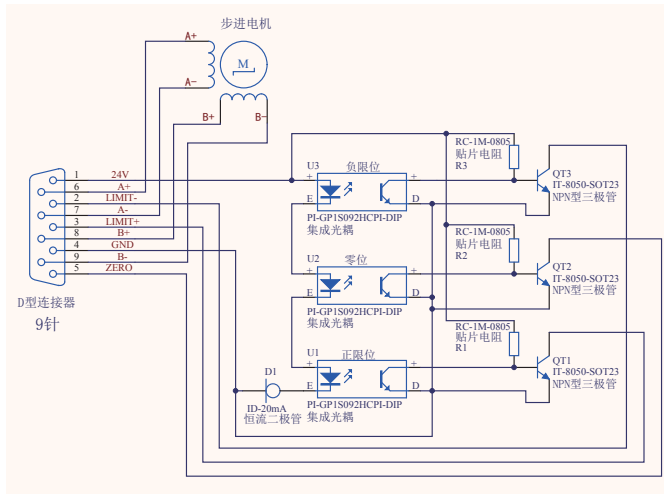
TBG45-60&TBG80-60
