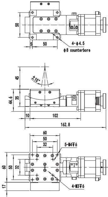
TBG100-80
